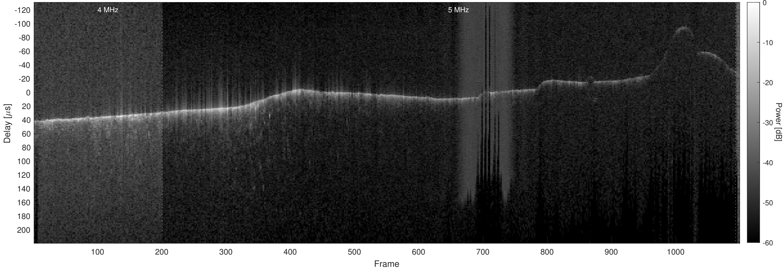
Orbit 9415, Optimized, No Window, Channel 2
