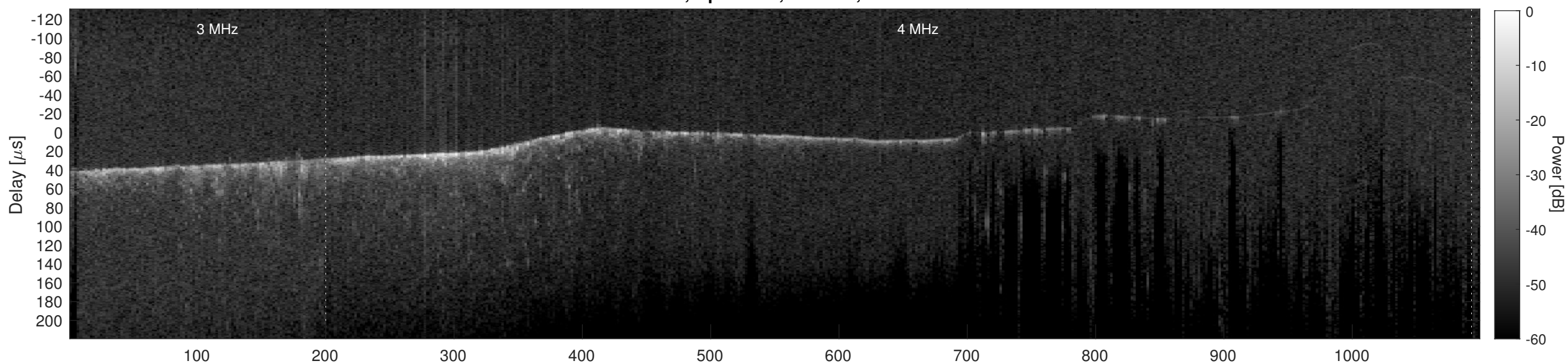
Orbit 9415, Cluttergram
