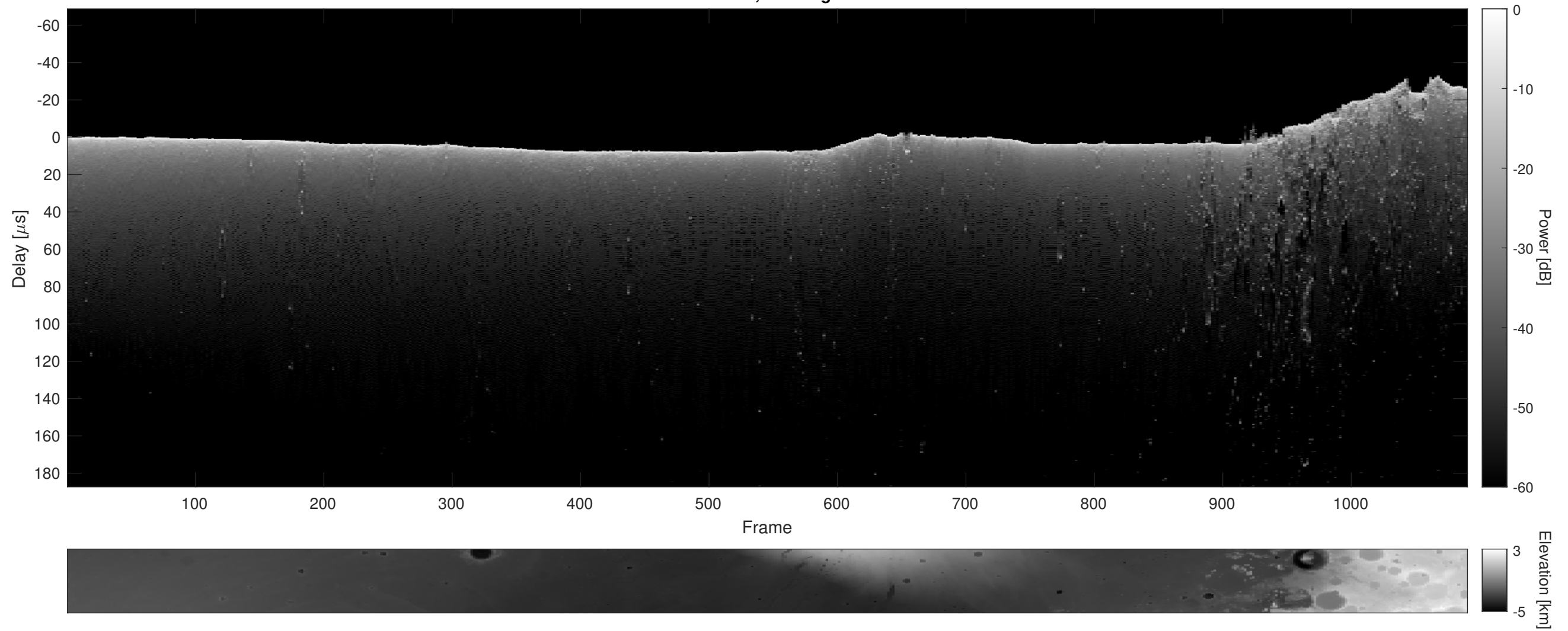
Orbit 9416, Cluttergram
