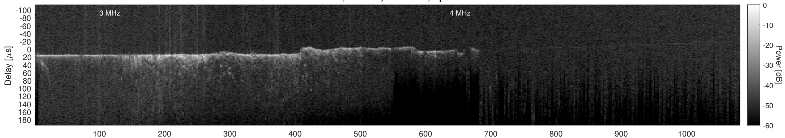
Orbit 9417, Cluttergram
