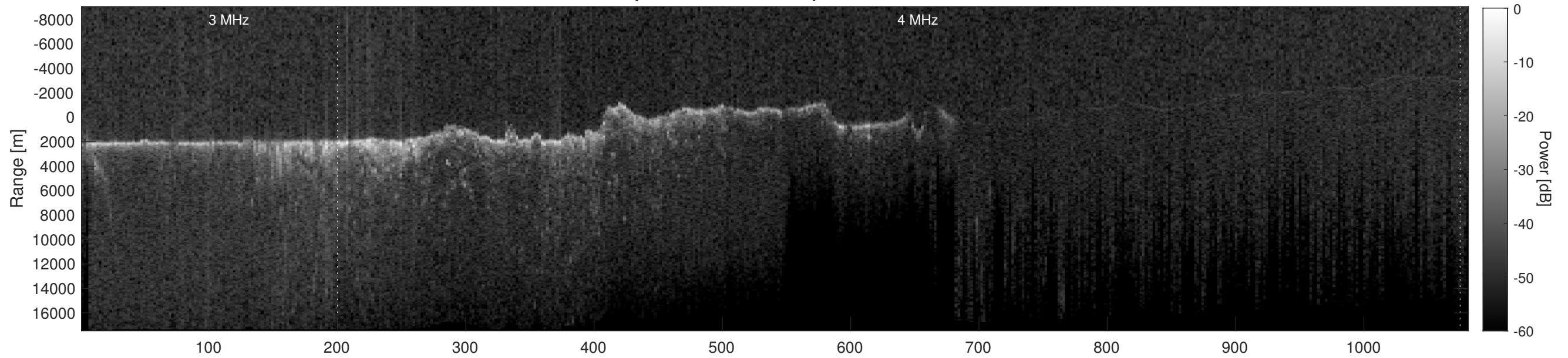
Orbit 9417, Depth-Corrected Cluttergram
