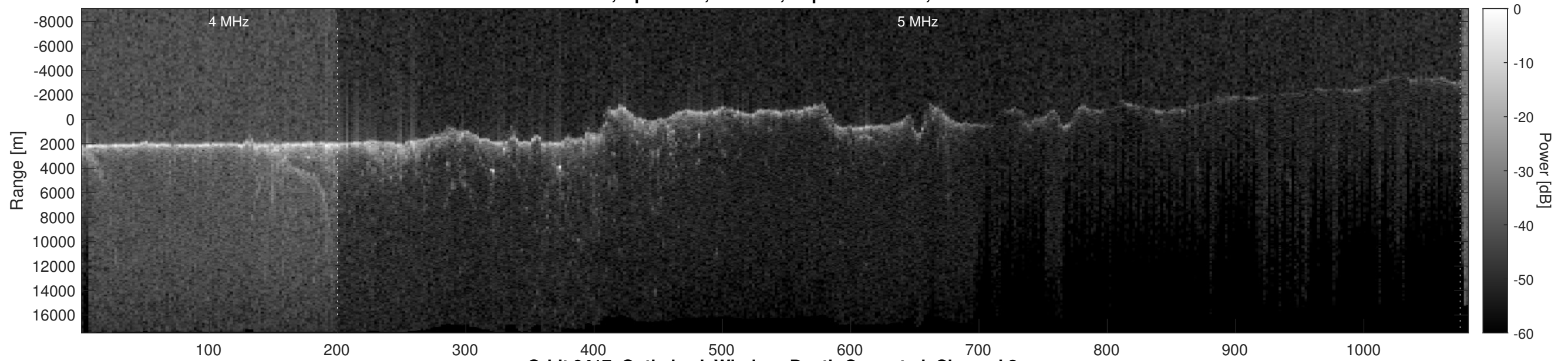
Orbit 9417, Optimized, Window, Depth-Corrected, Channel 2
