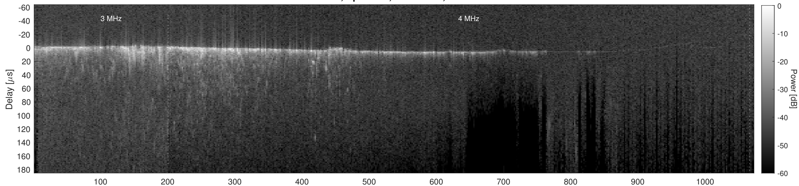
Orbit 9419, Cluttergram
