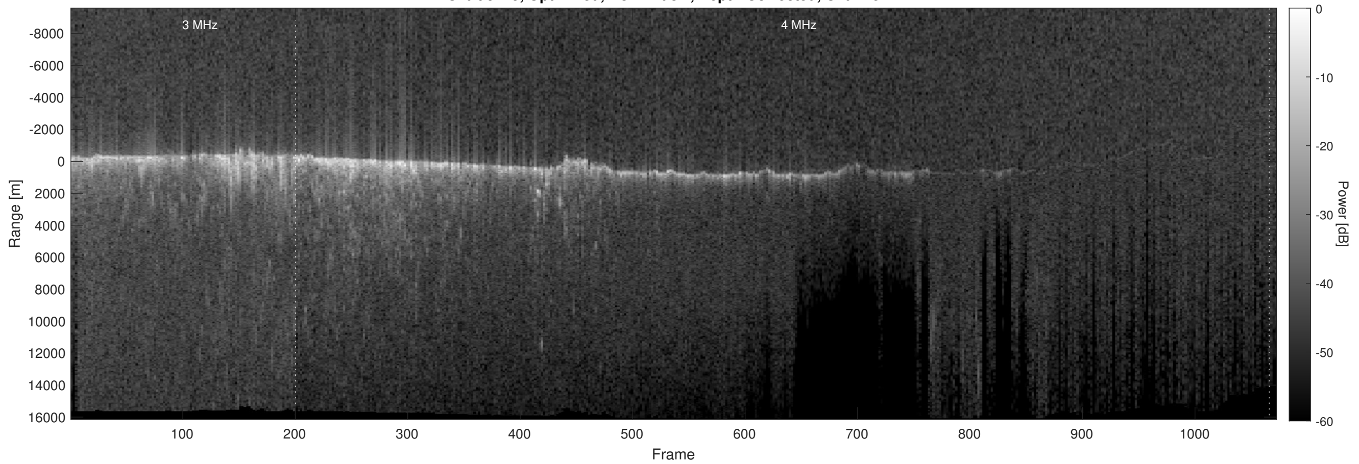
Orbit 9419, Optimized, No Window, Depth-Corrected, Channel 2
