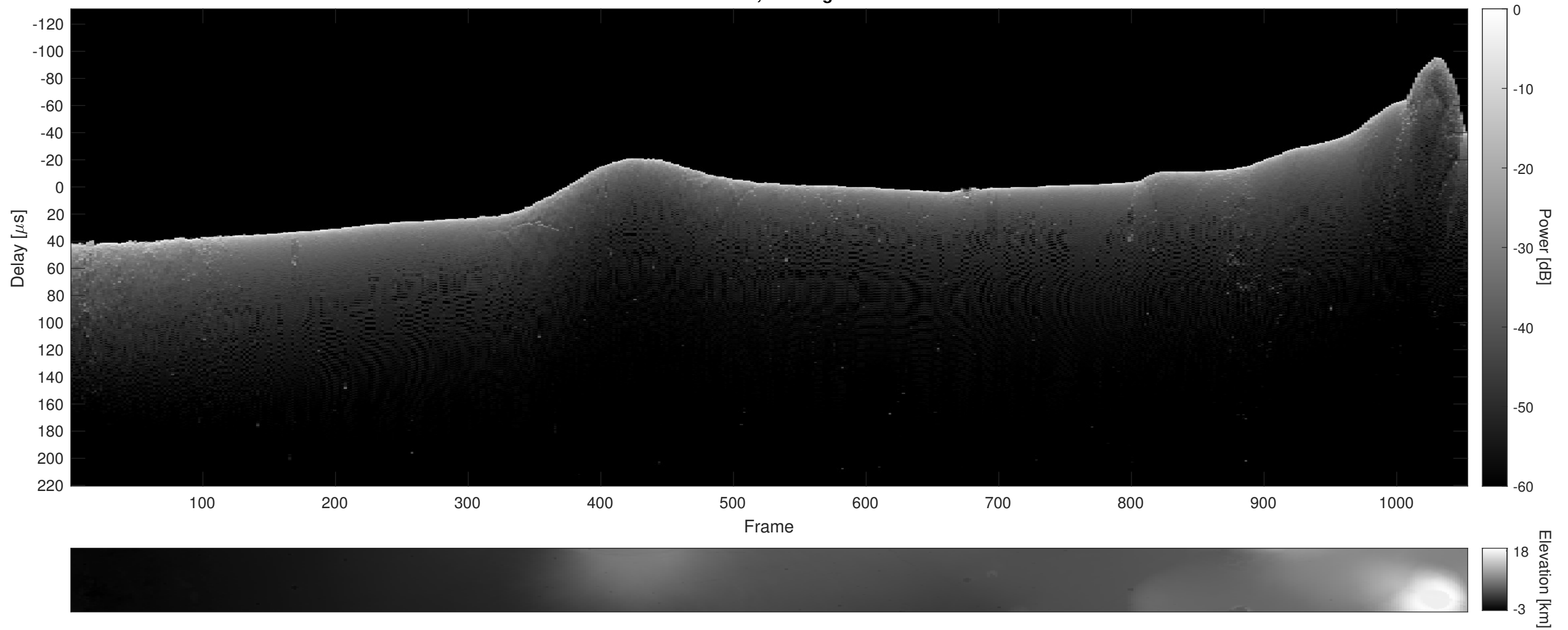
Orbit 9422, Cluttergram
