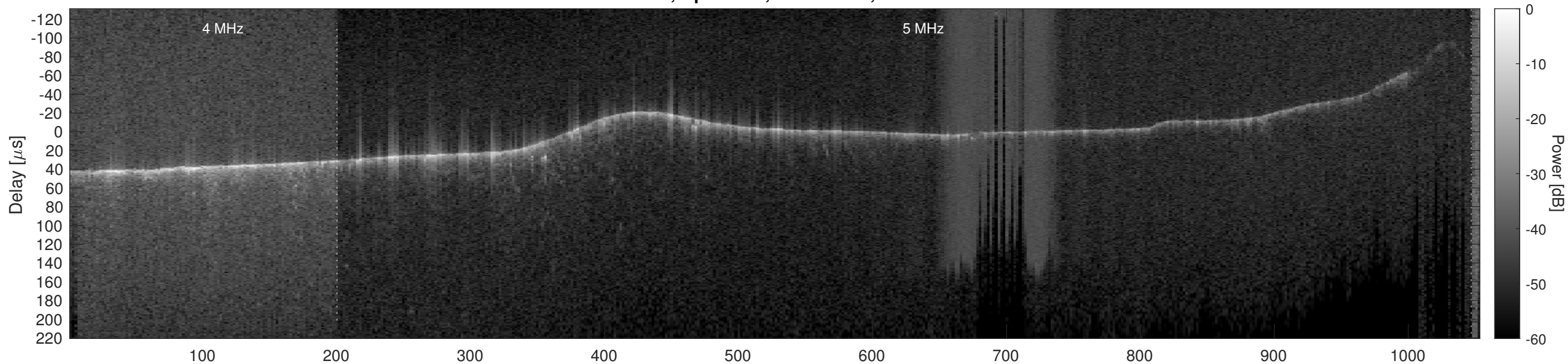
Orbit 9422, Optimized, No Window, Channel 2
