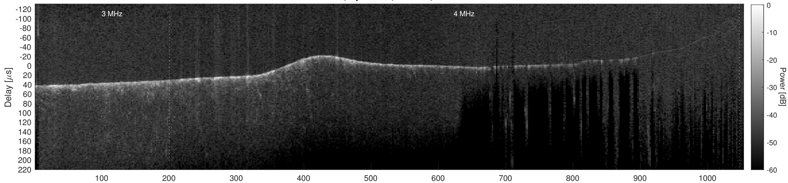
Orbit 9422, Cluttergram
