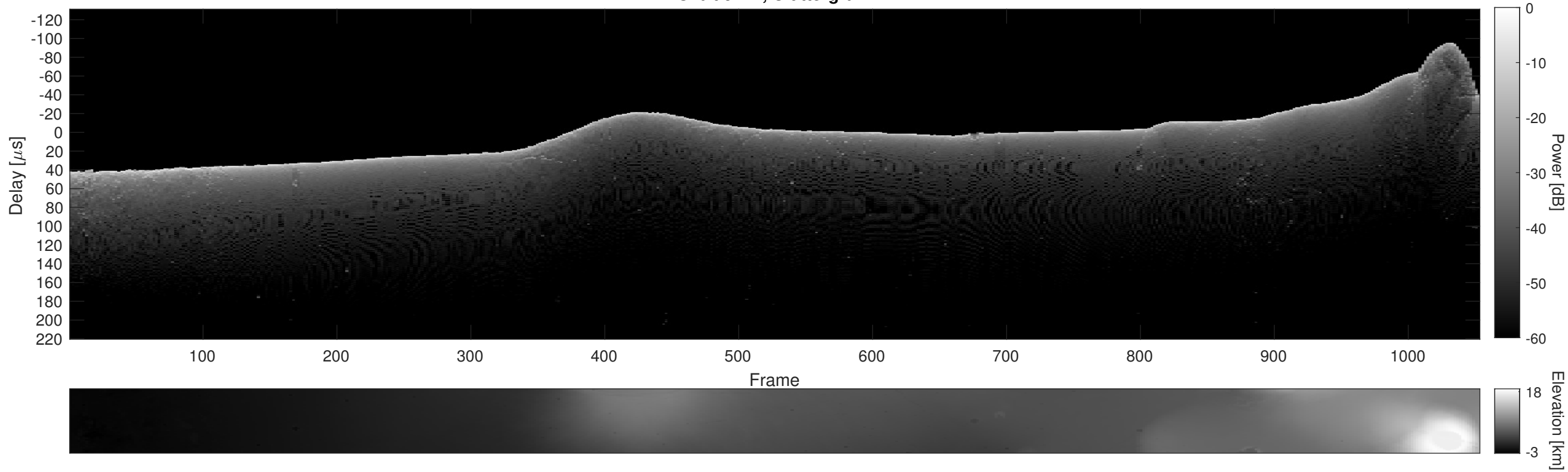
Orbit 9422, Cluttergram
