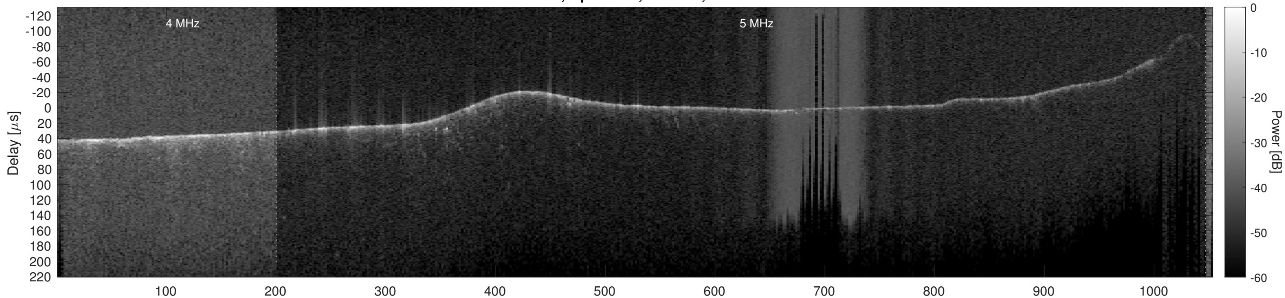
Orbit 9422, Optimized, Window, Channel 2
