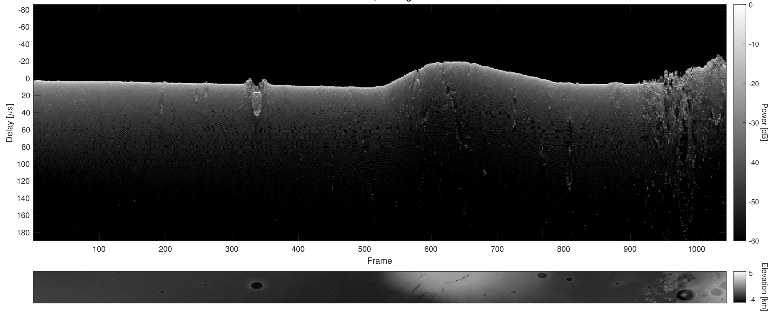
Orbit 9423, Cluttergram
