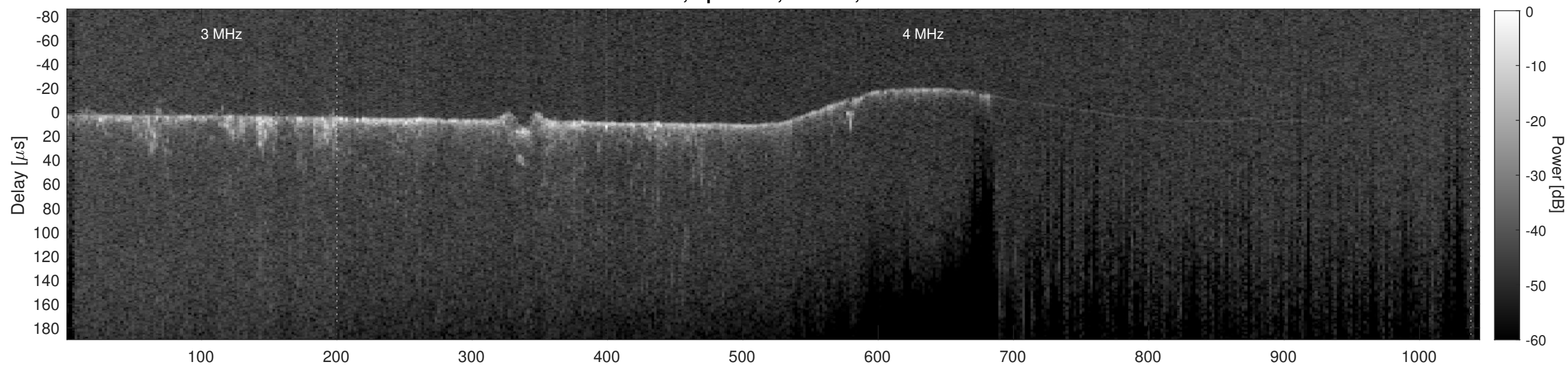
Orbit 9423, Cluttergram
