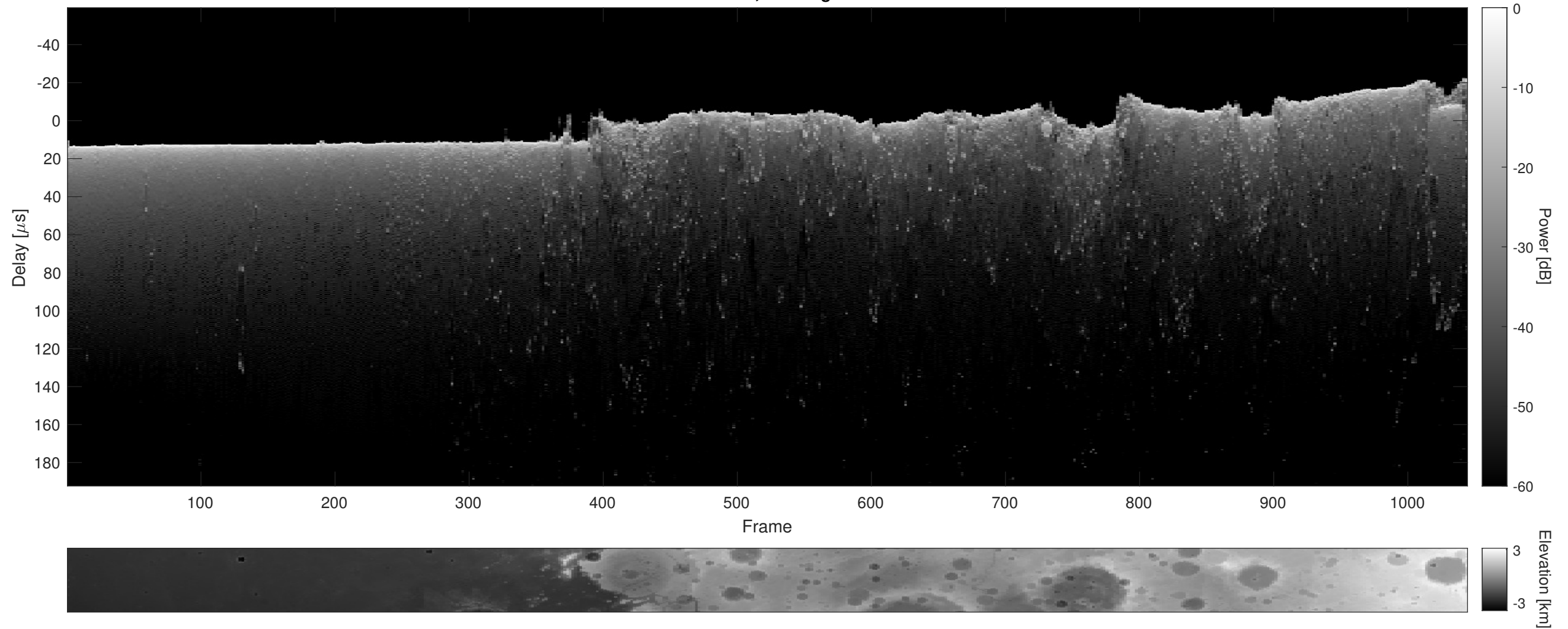
Orbit 9424, Cluttergram
