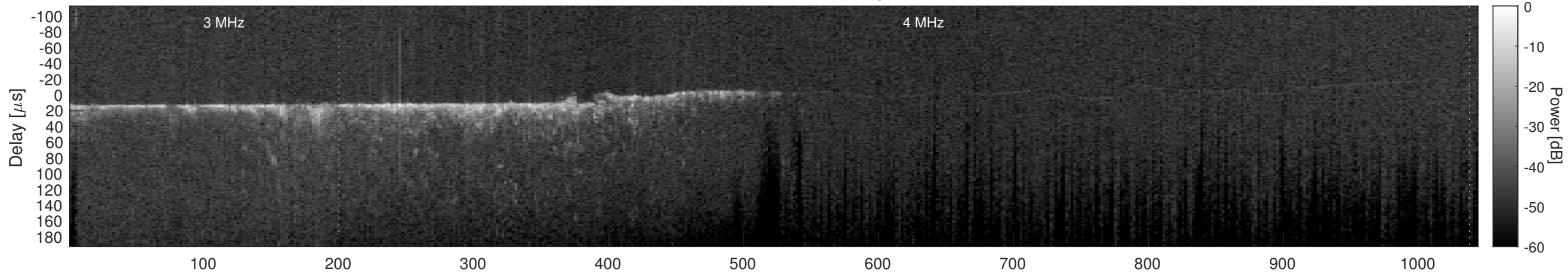
Orbit 9424, Cluttergram
