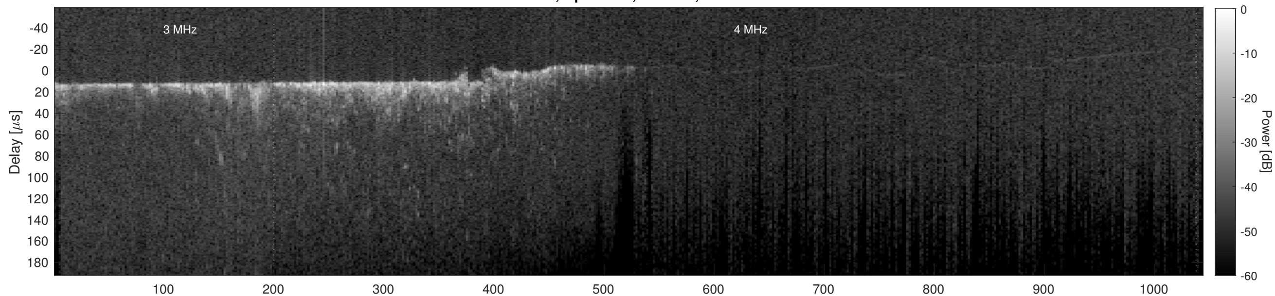
Orbit 9424, Cluttergram
