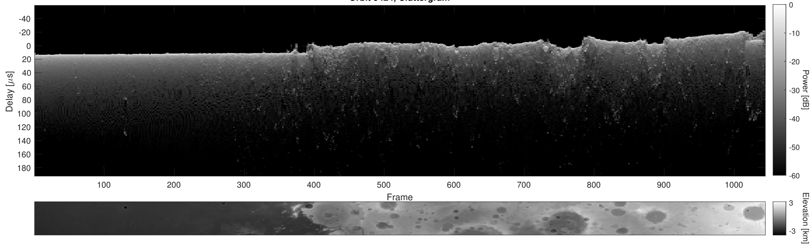
Orbit 9424, Cluttergram
