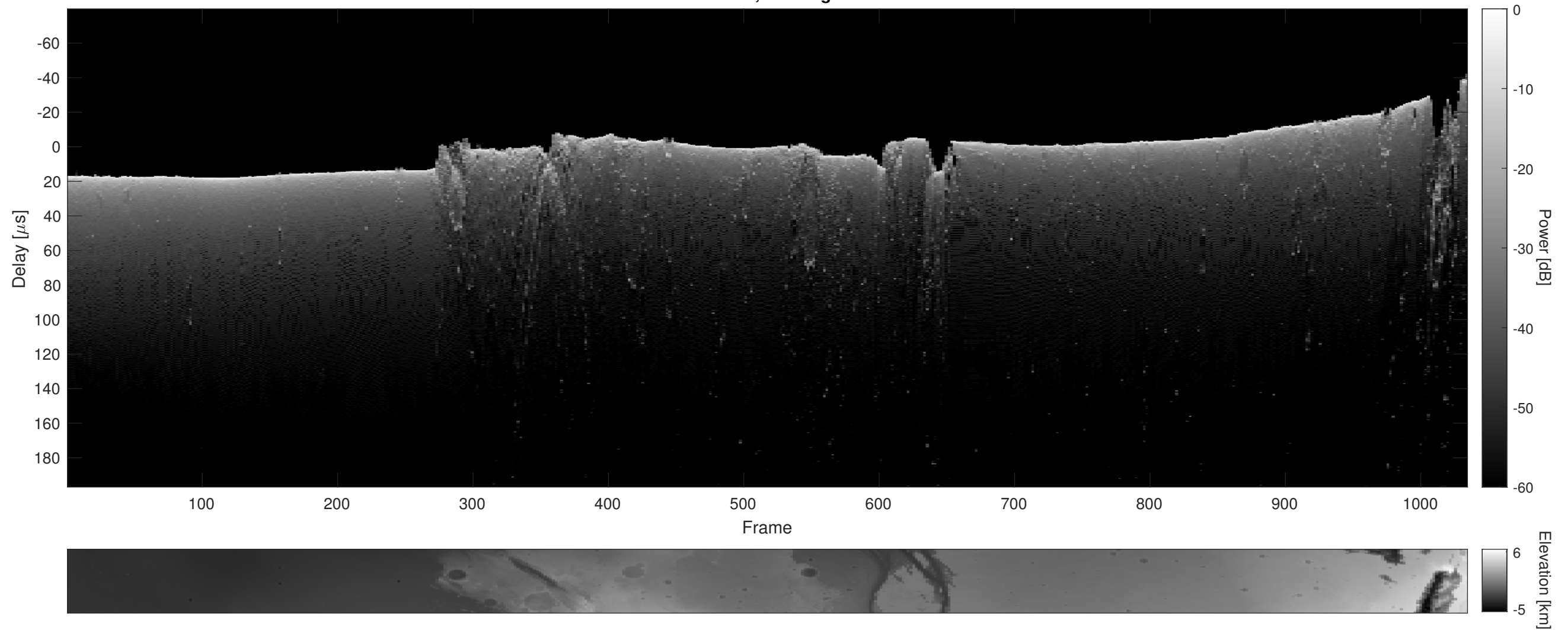
Orbit 9425, Cluttergram
