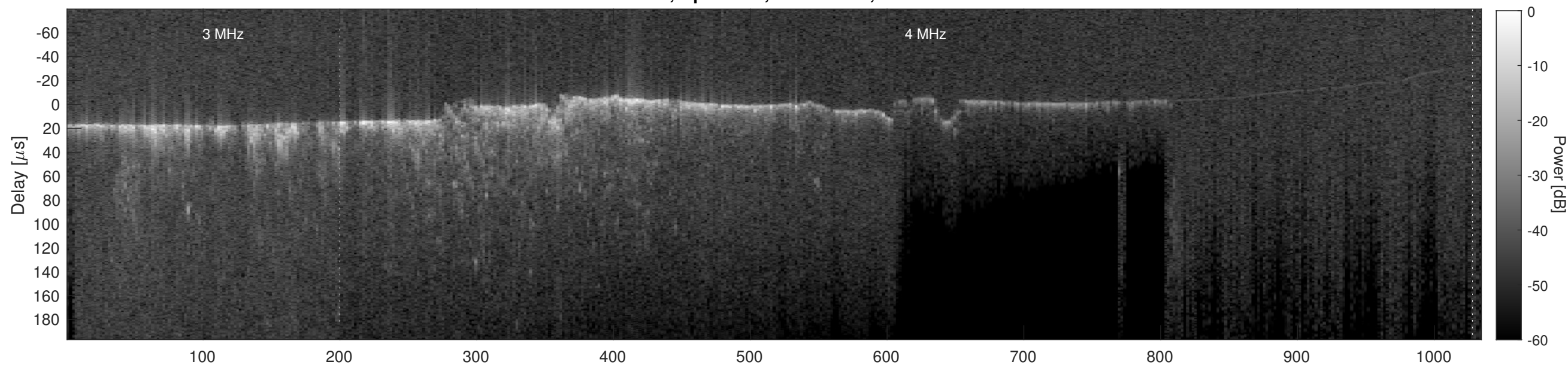
Orbit 9425, Cluttergram
