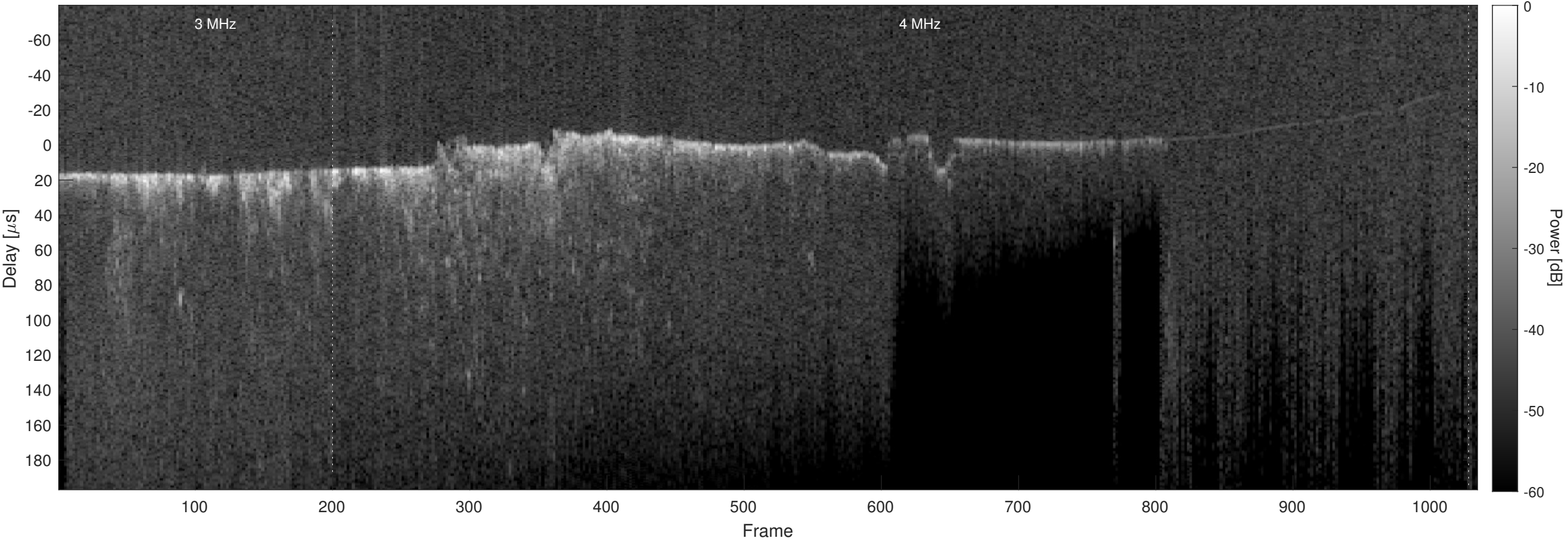
Orbit 9425, Optimized, Window, Channel 2
