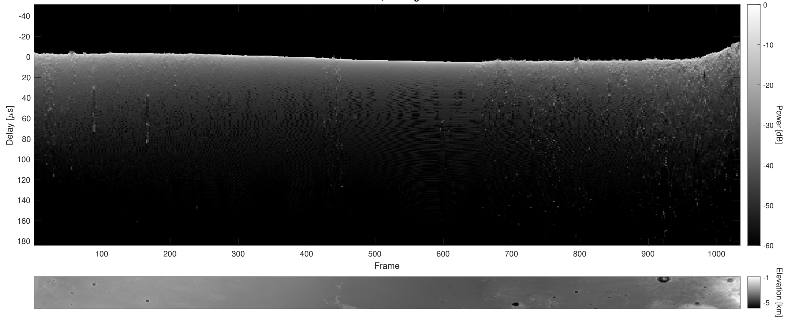
Orbit 9426, Cluttergram
