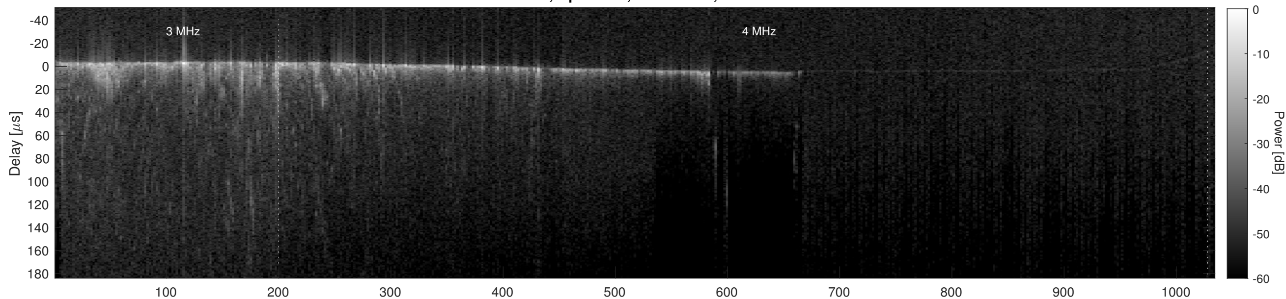
Orbit 9426, Cluttergram
