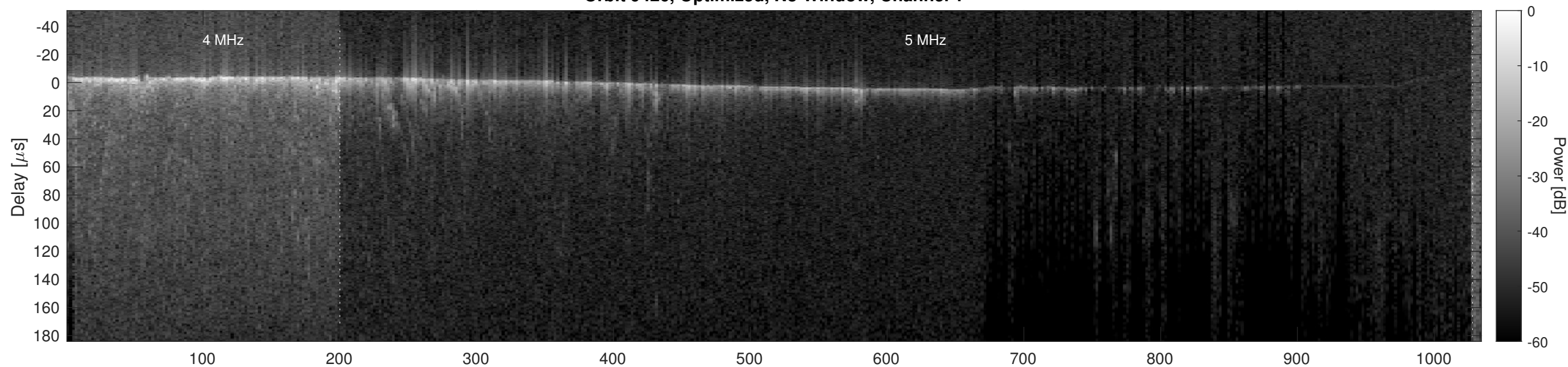
Orbit 9426, Optimized, No Window, Channel 2
