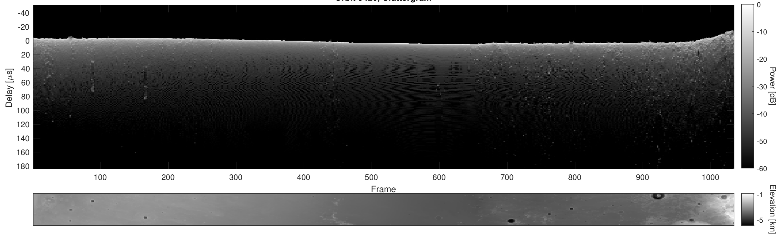
Orbit 9426, Cluttergram
