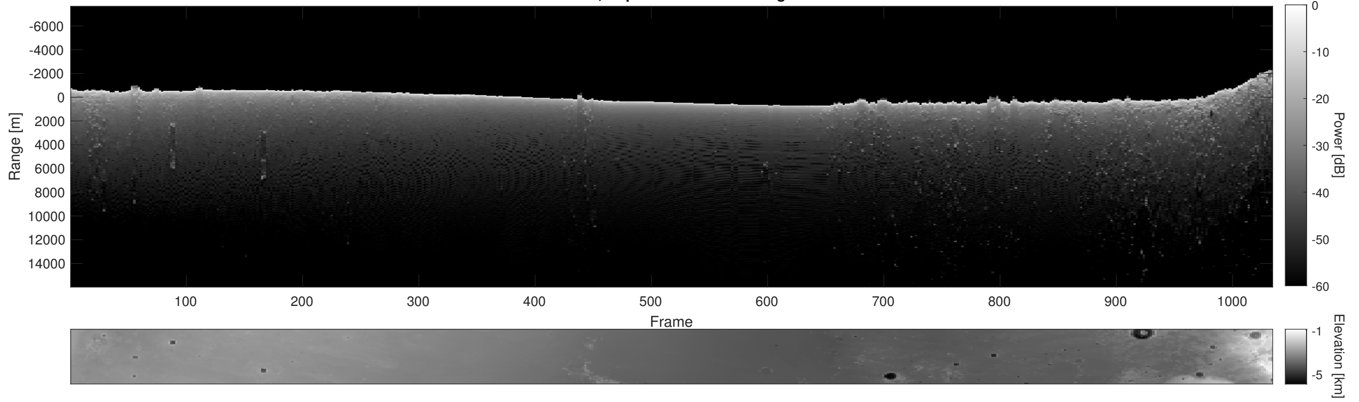
Orbit 9426, Depth-Corrected Cluttergram
