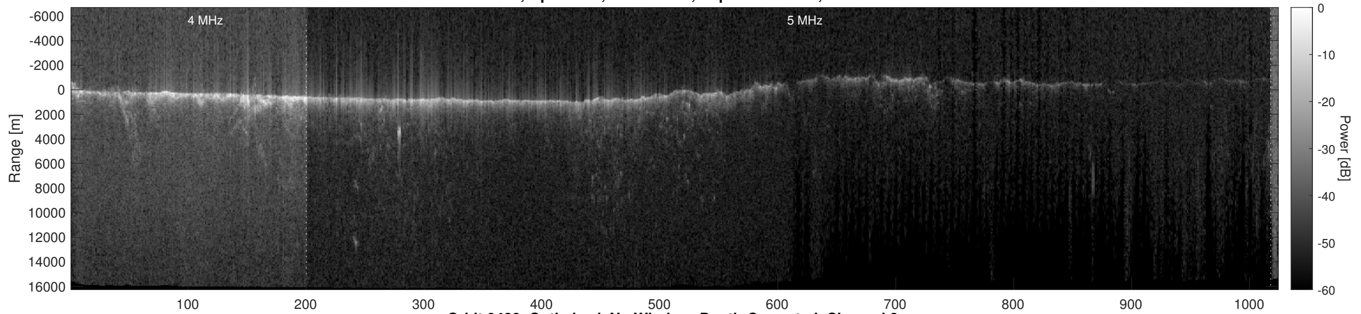
Orbit 9428, Optimized, No Window, Depth-Corrected, Channel 2
