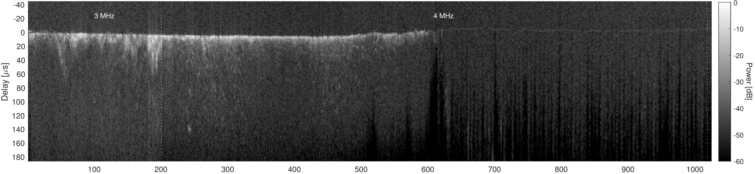
Orbit 9428, Cluttergram
