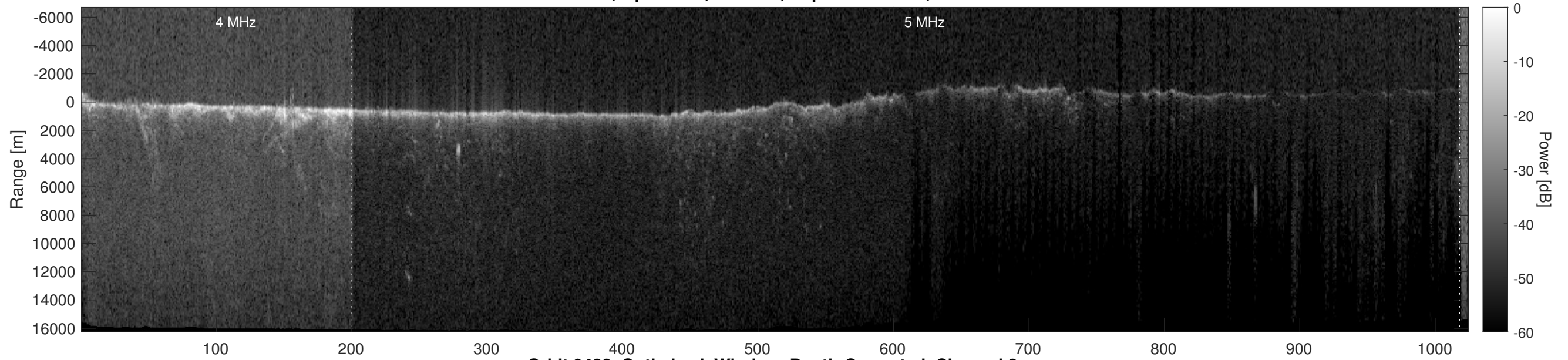
Orbit 9428, Optimized, Window, Depth-Corrected, Channel 2
