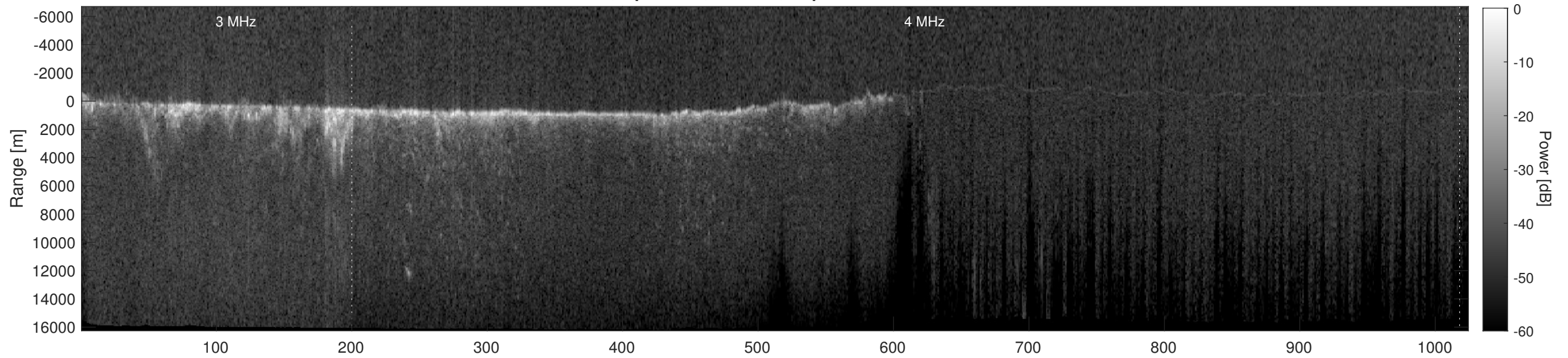
Orbit 9428, Depth-Corrected Cluttergram
