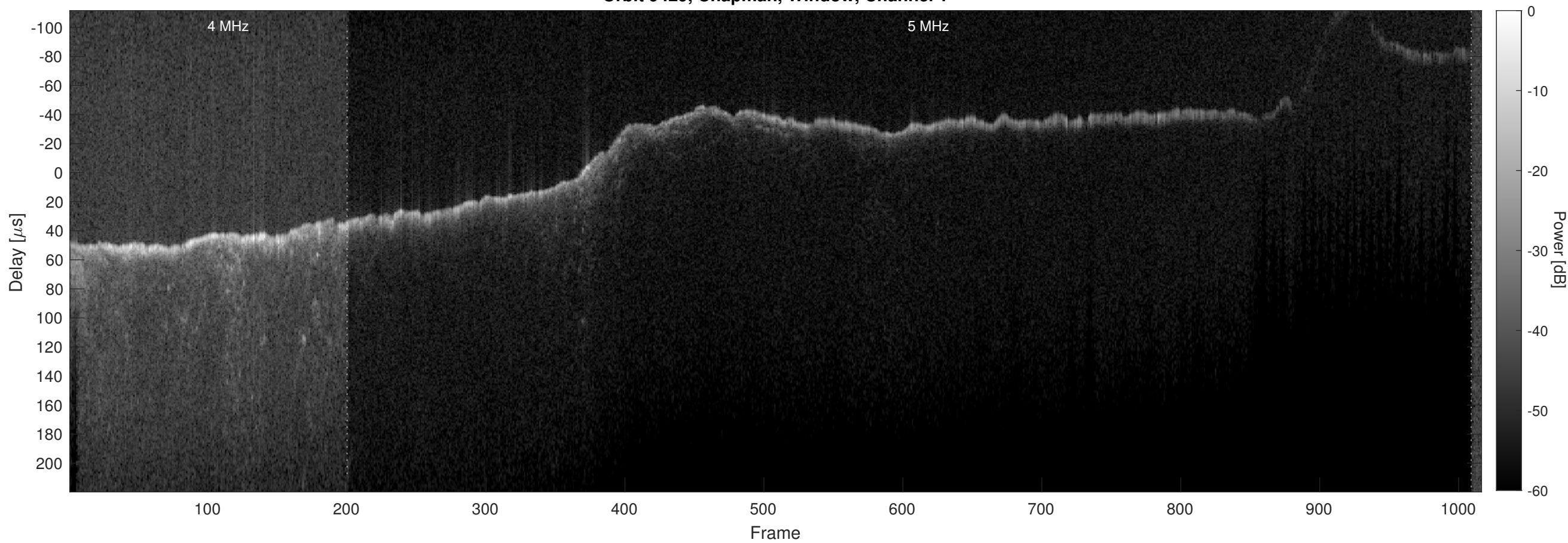
Orbit 9429, Chapman, Window, Channel 2
