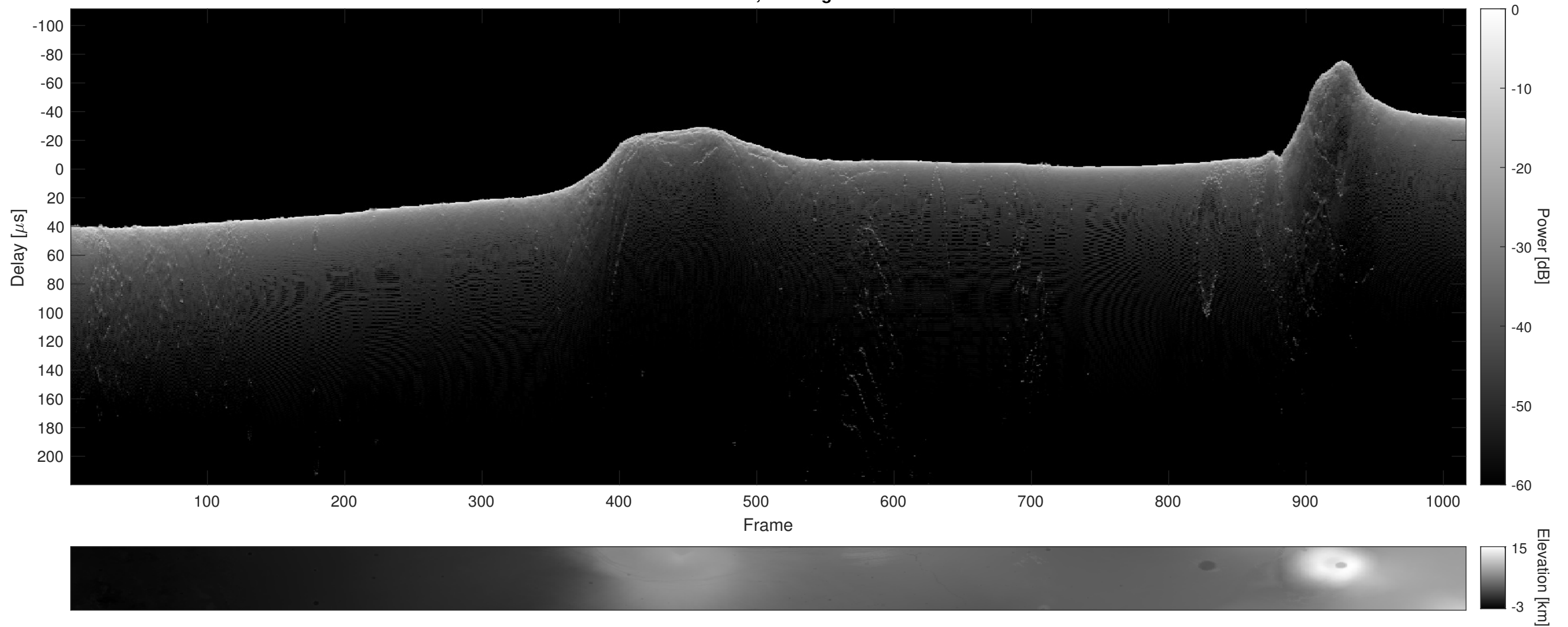
Orbit 9429, Cluttergram
