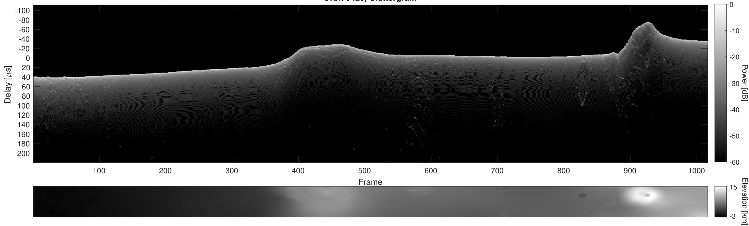
Orbit 9429, Cluttergram
