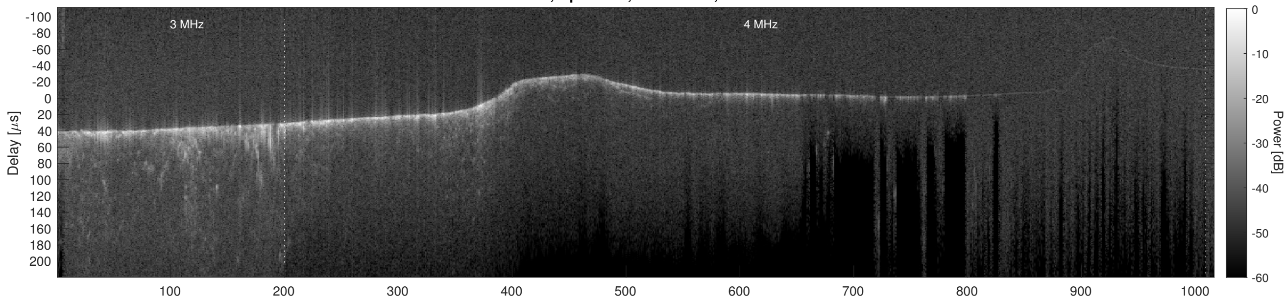
Orbit 9429, Cluttergram
