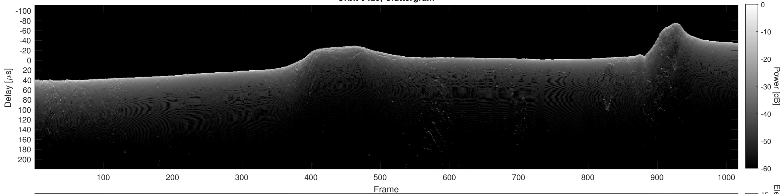
Orbit 9429, Cluttergram
