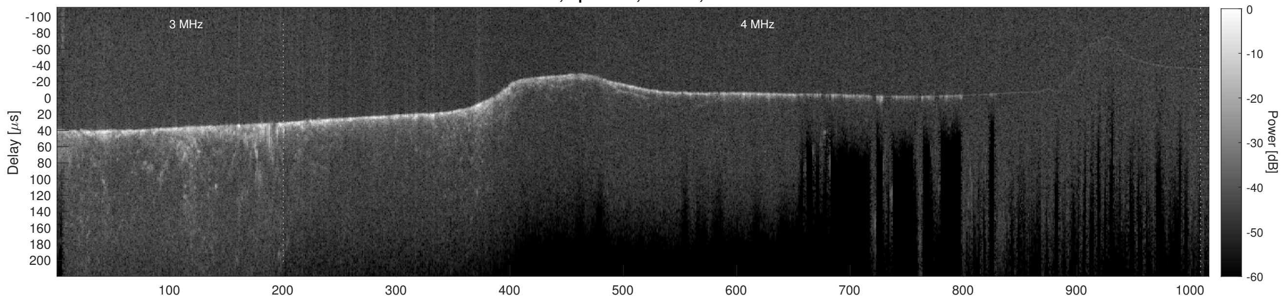
Orbit 9429, Cluttergram
