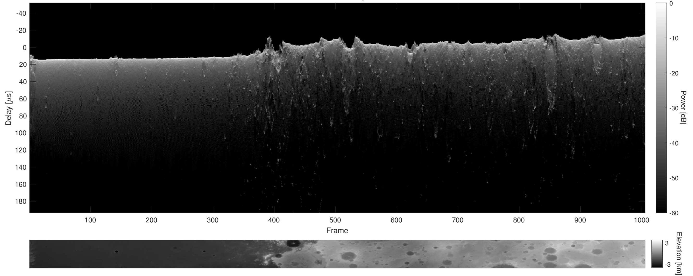
Orbit 9431, Cluttergram
