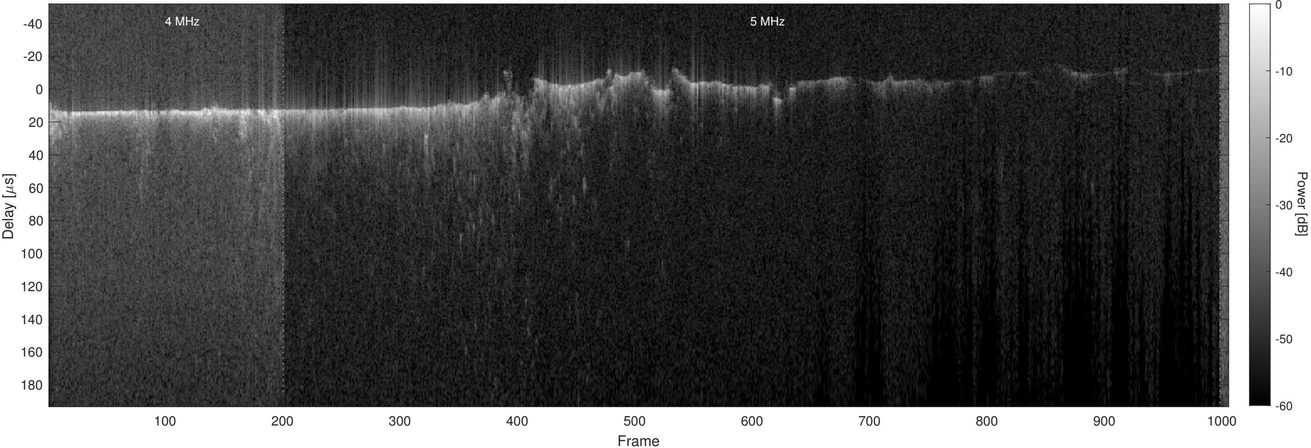
Orbit 9431, Optimized, No Window, Channel 2
