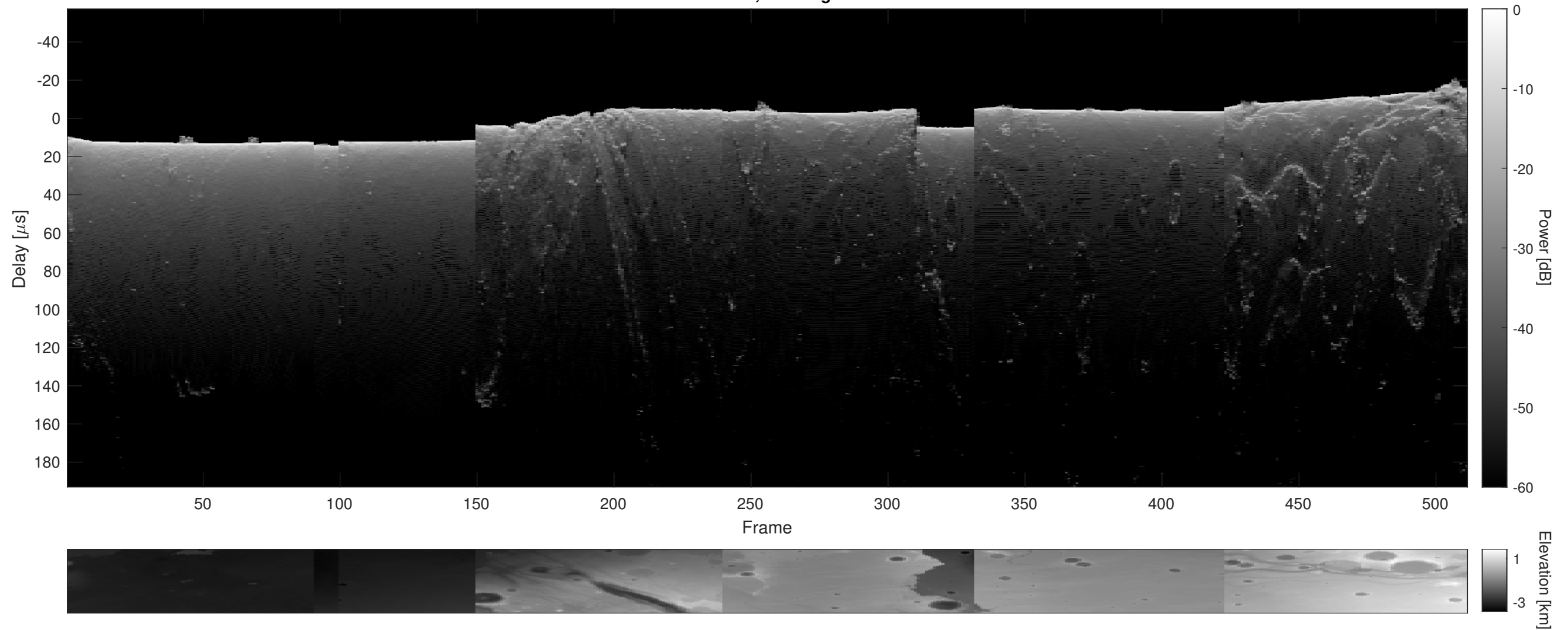
Orbit 9432, Cluttergram
