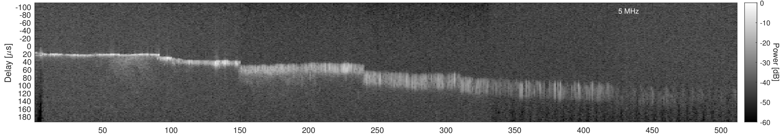
Orbit 9432, Window, Channel 2, Chapman
