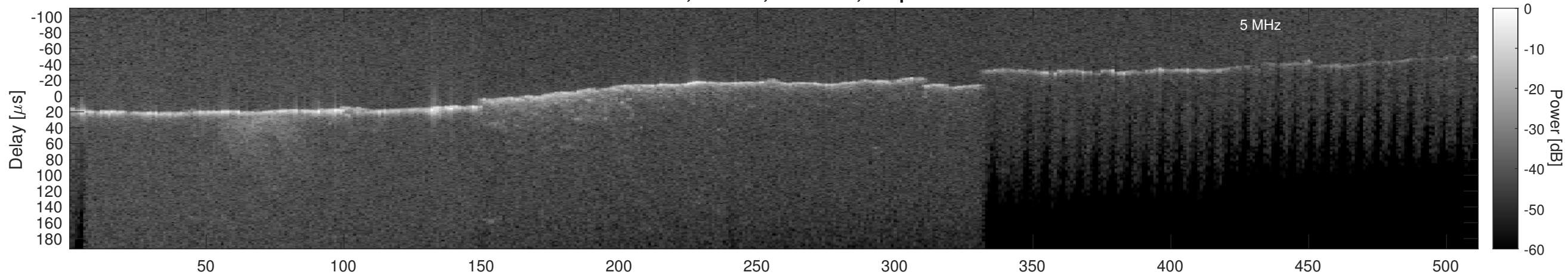
Orbit 9432, Window, Channel 2, Optimized
