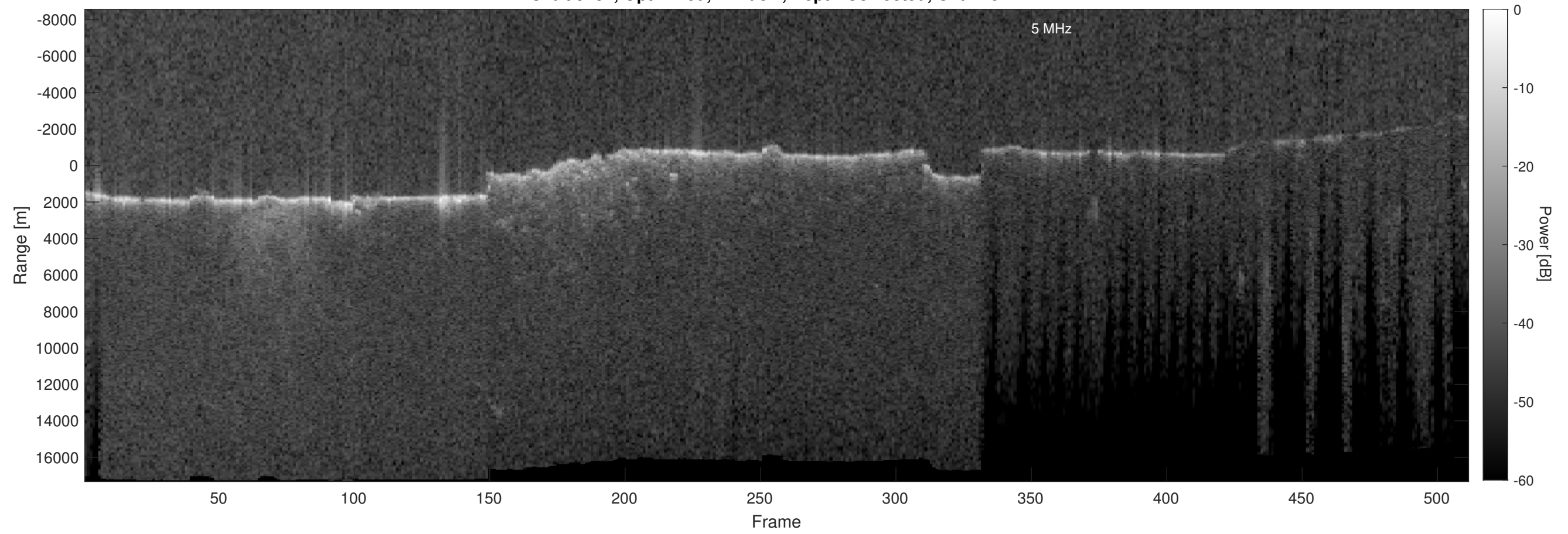
Orbit 9432, Optimized, Window, Depth-Corrected, Channel 2
