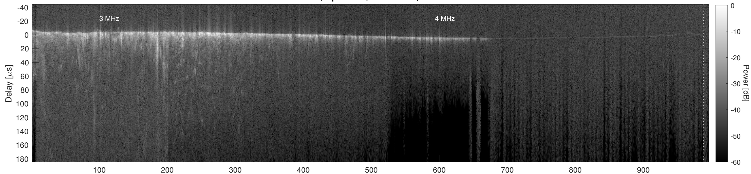
Orbit 9433, Cluttergram
