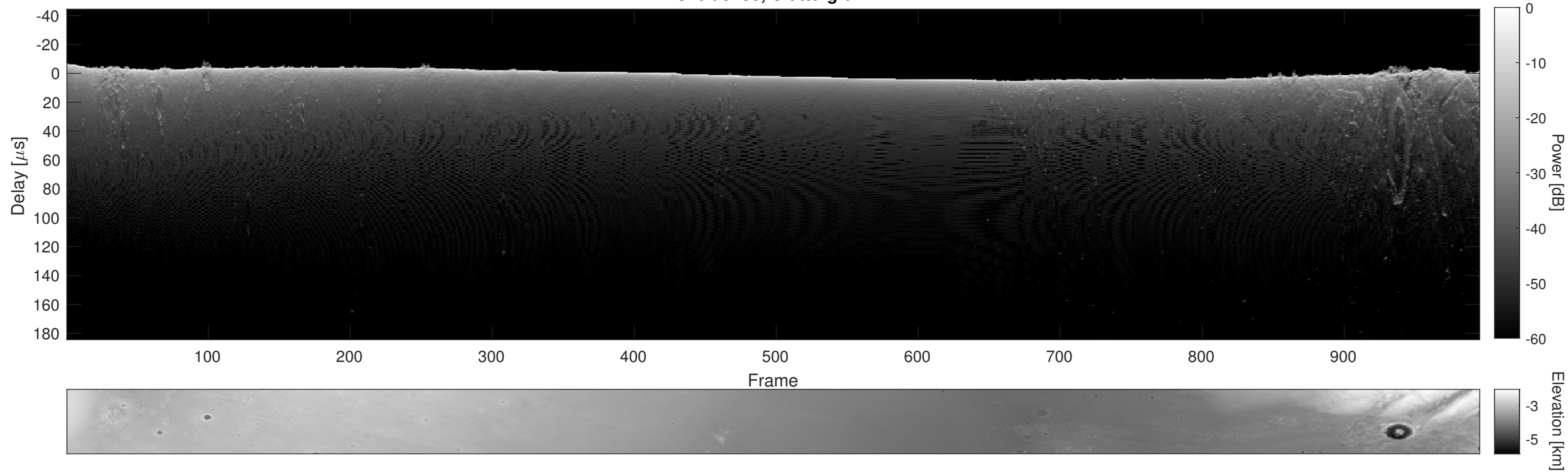
Orbit 9433, Cluttergram
