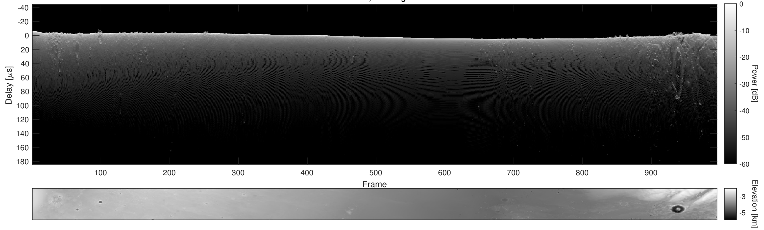
Orbit 9433, Cluttergram
