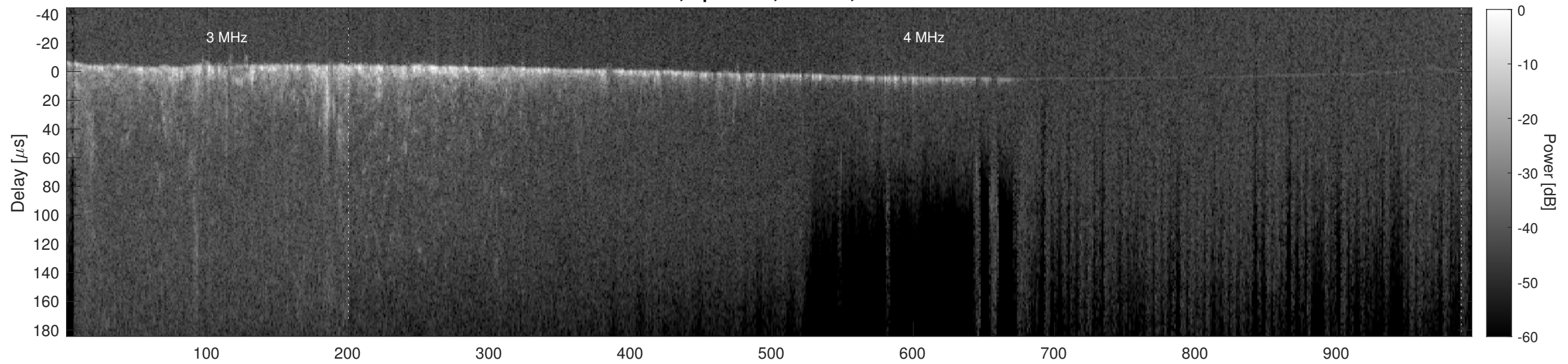
Orbit 9433, Cluttergram
