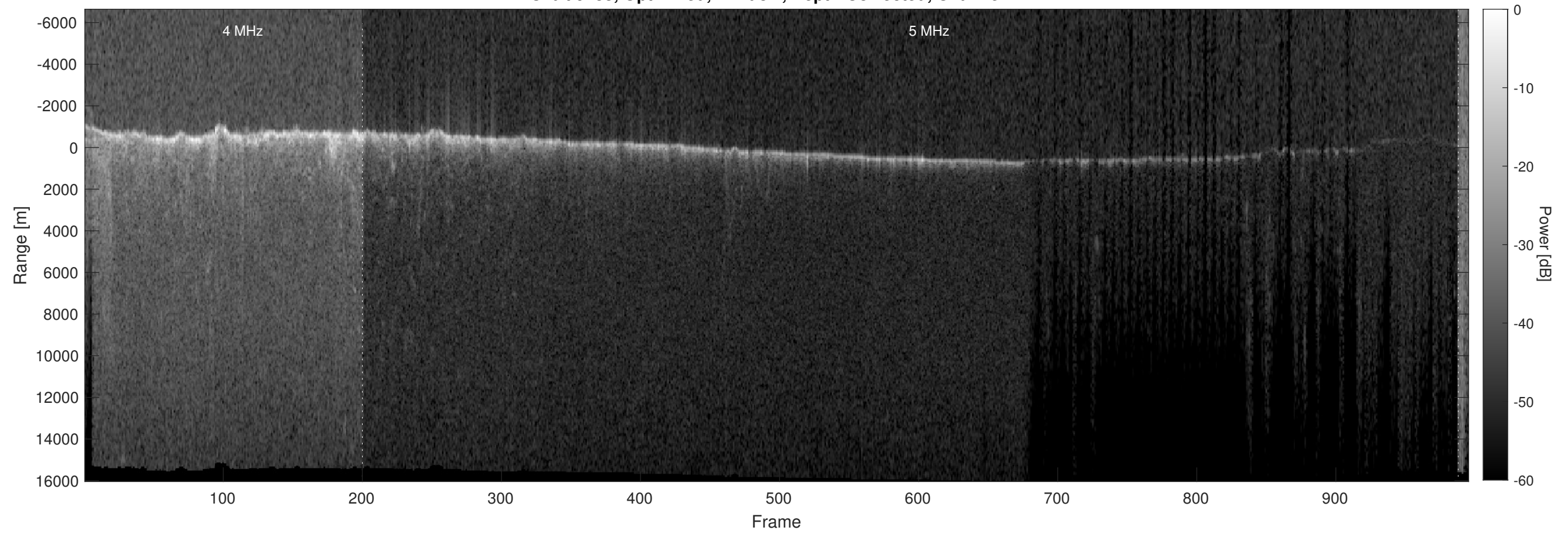
Orbit 9433, Optimized, Window, Depth-Corrected, Channel 2
