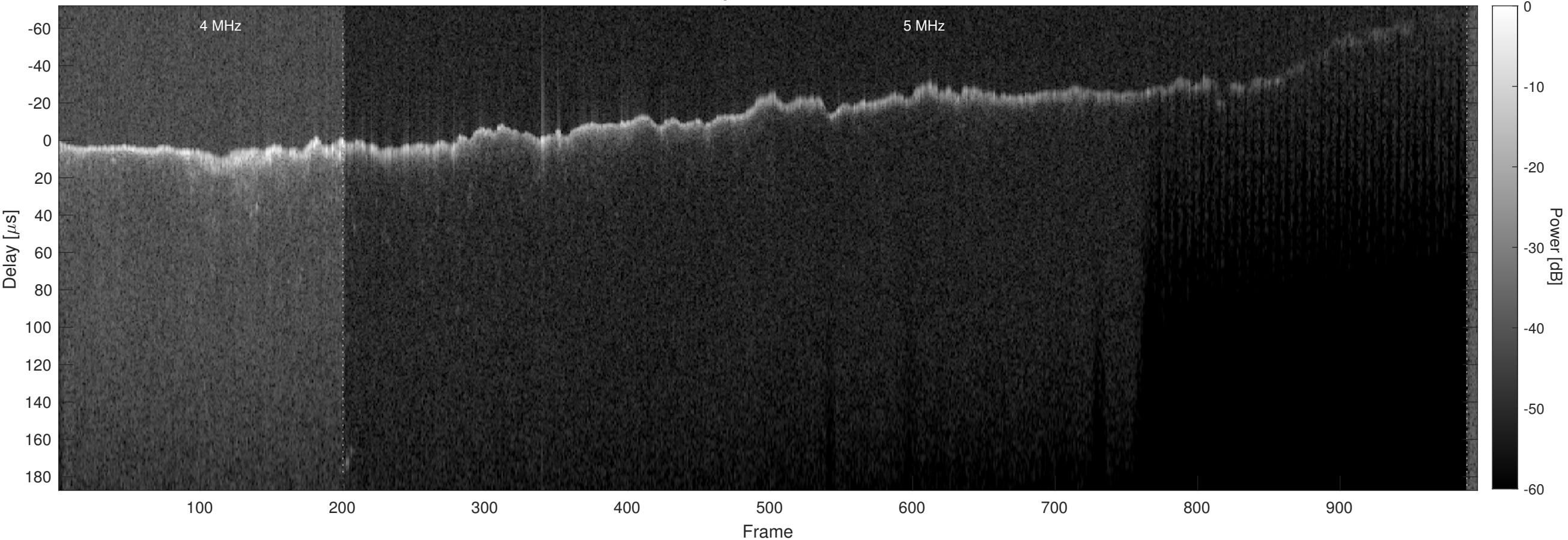
Orbit 9434, Chapman, Window, Channel 2
