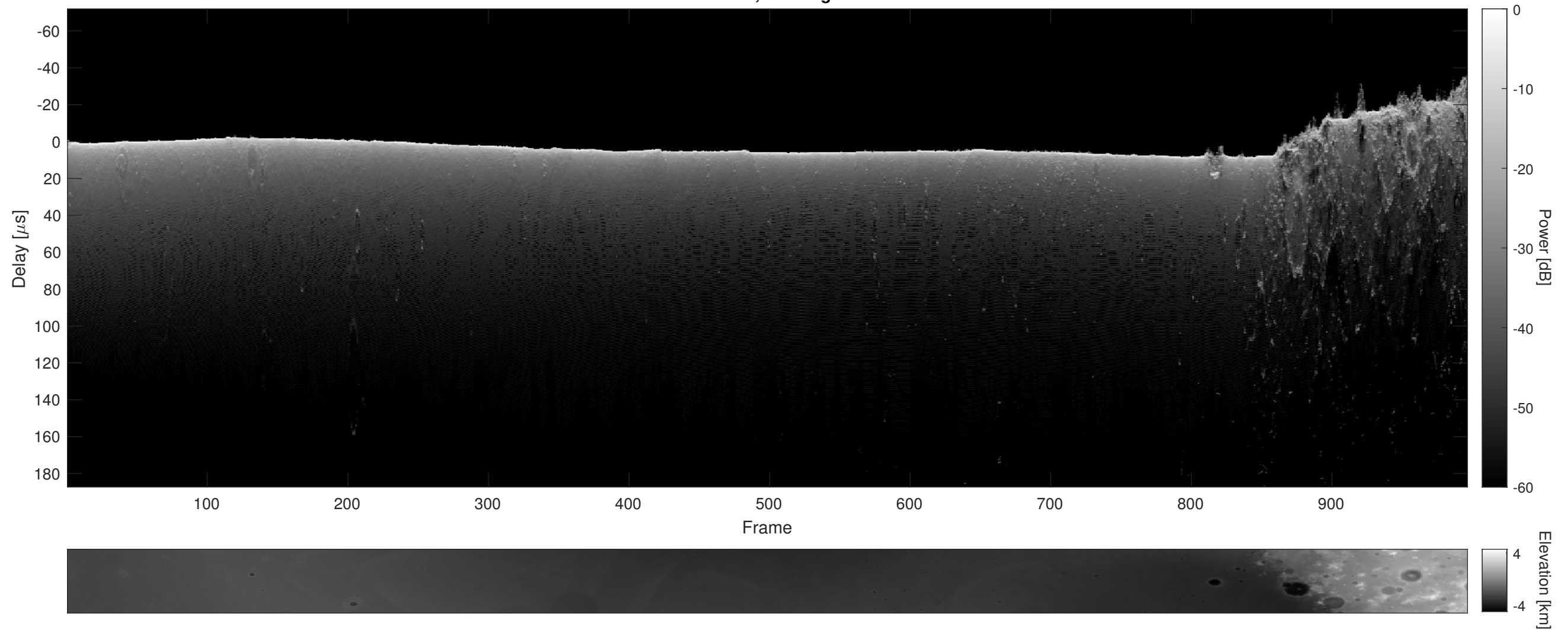
Orbit 9434, Cluttergram
