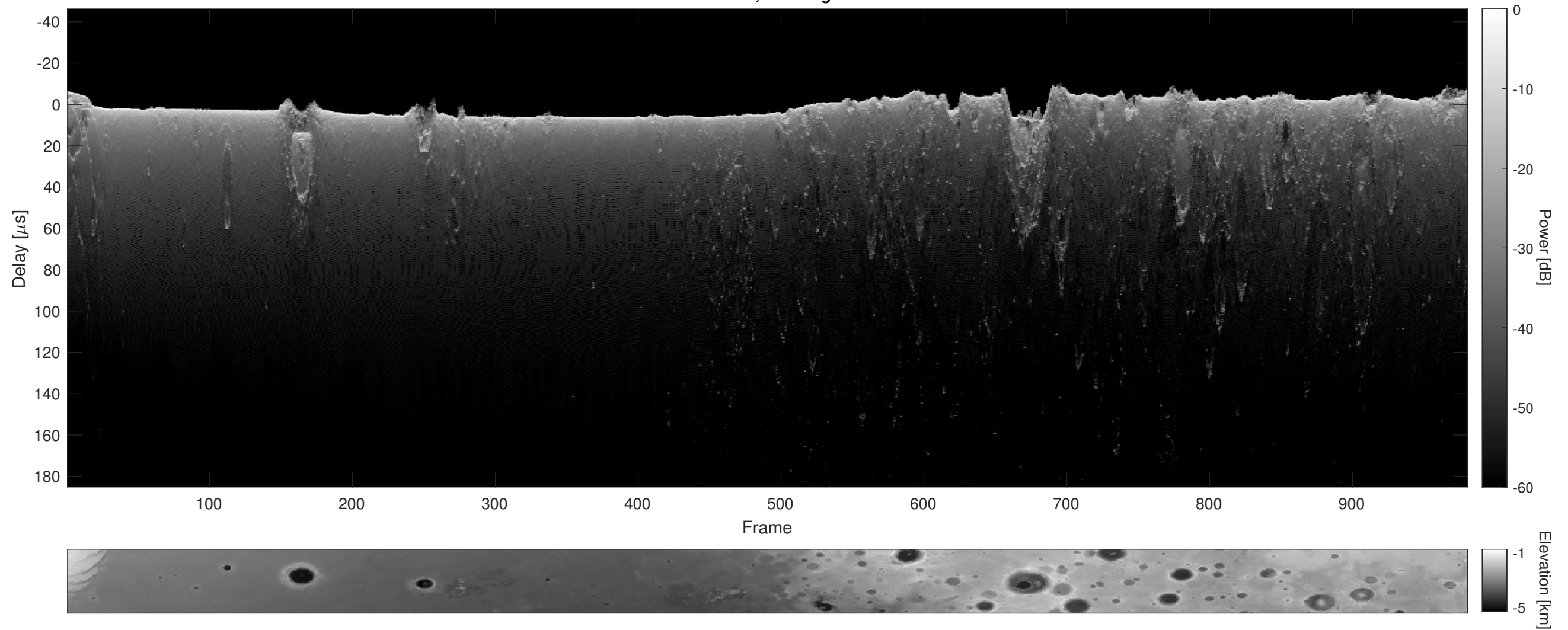
Orbit 9435, Cluttergram
