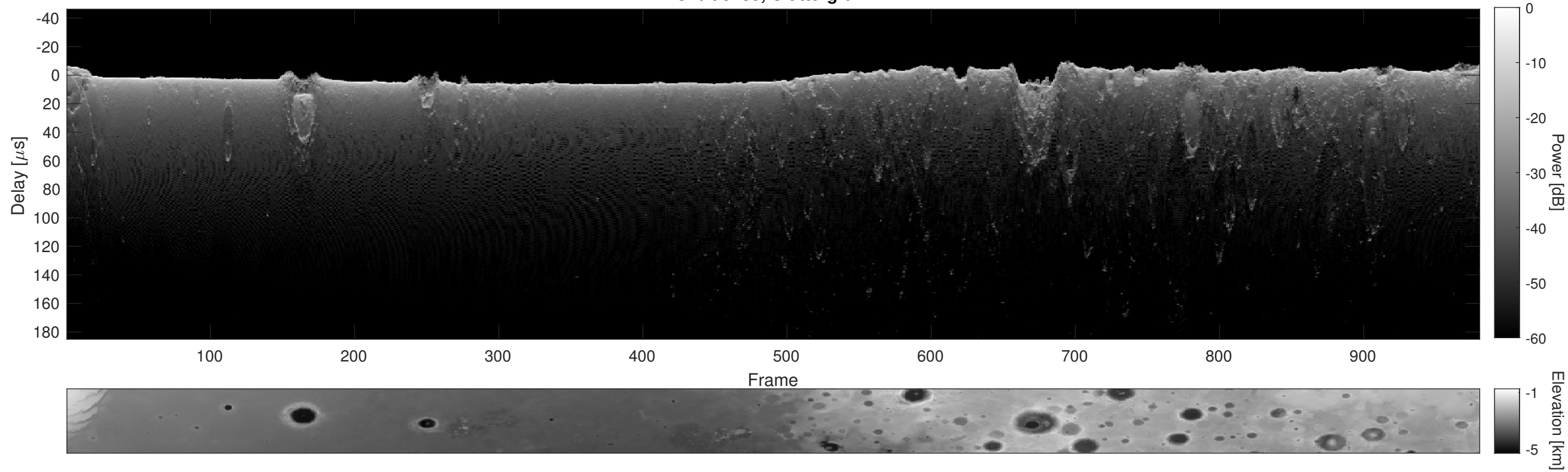
Orbit 9435, Cluttergram
