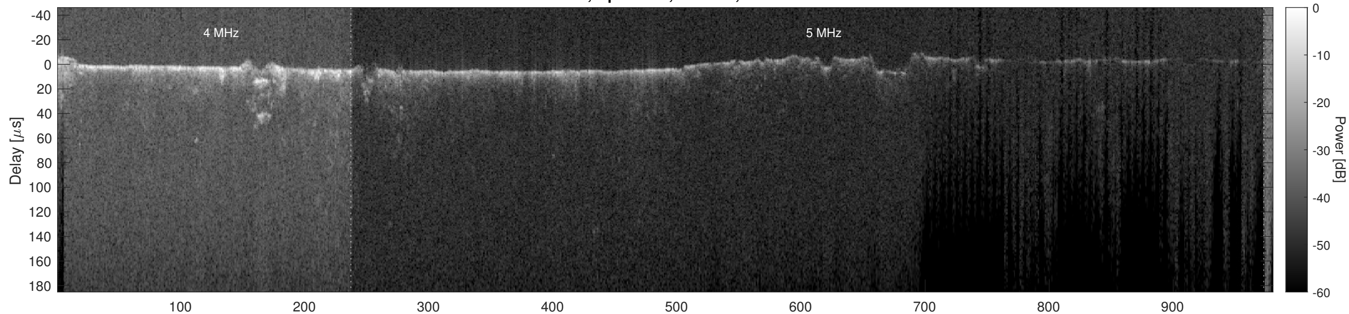
Orbit 9435, Optimized, Window, Channel 2
