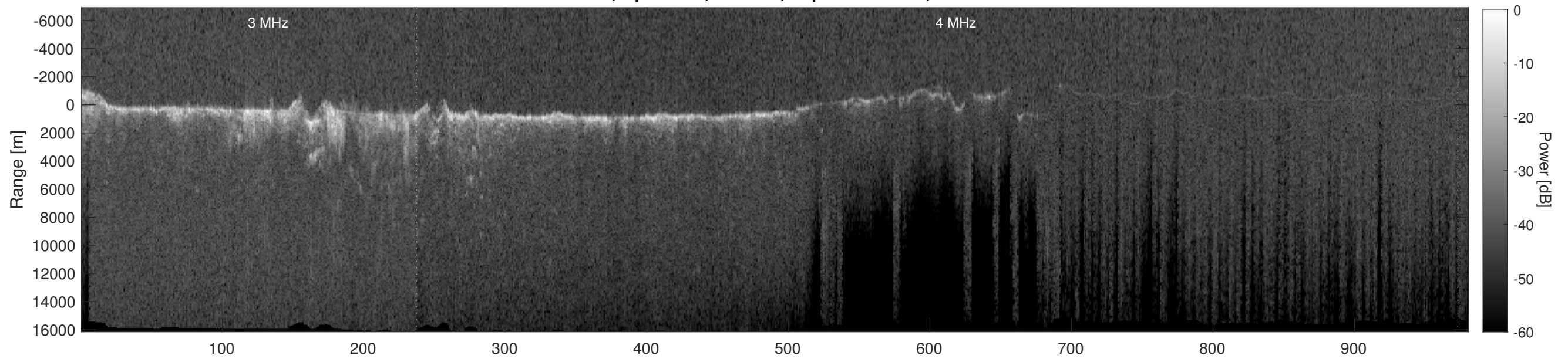
Orbit 9435, Depth-Corrected Cluttergram
