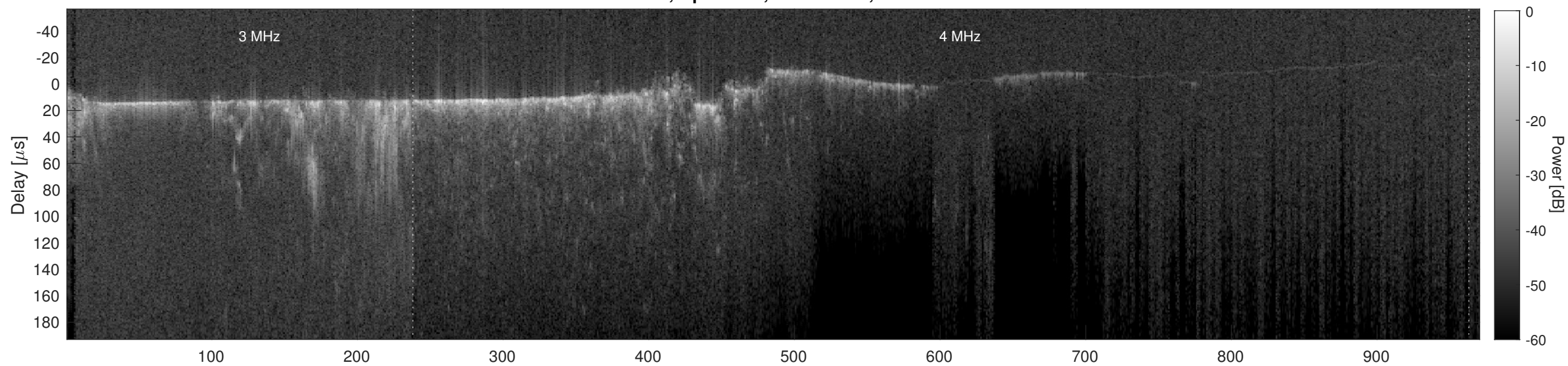
Orbit 9438, Cluttergram
