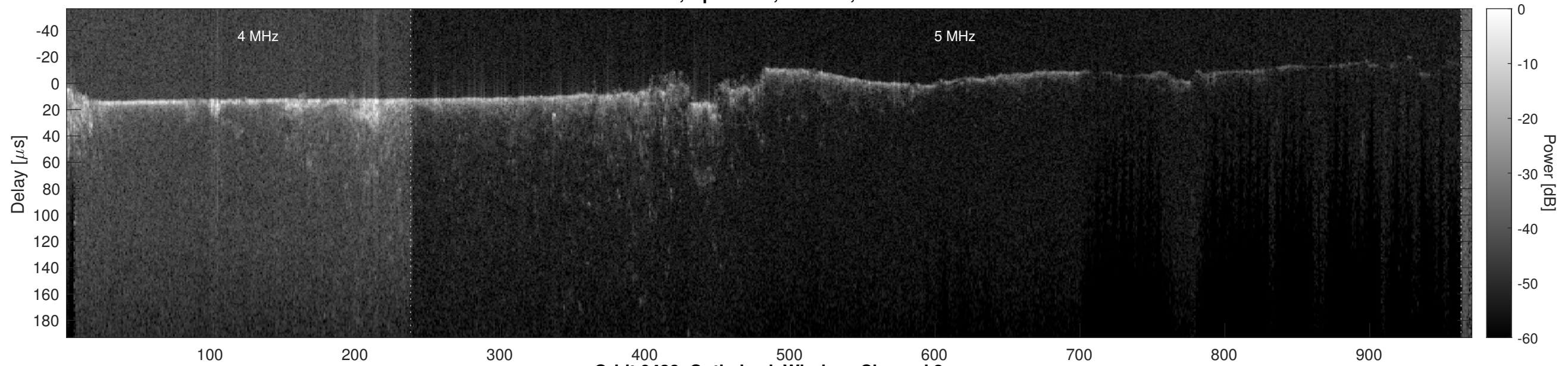
Orbit 9438, Optimized, Window, Channel 2
