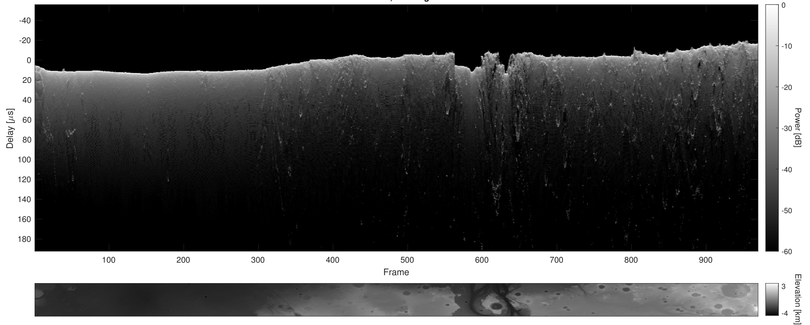
Orbit 9439, Cluttergram
