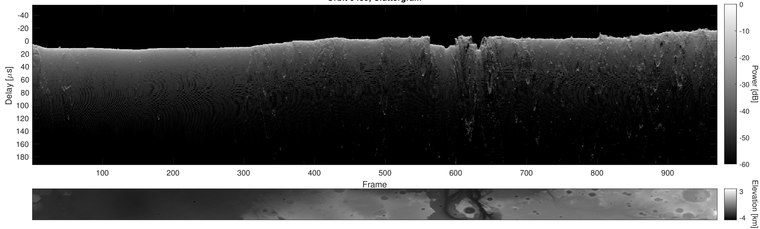
Orbit 9439, Cluttergram
