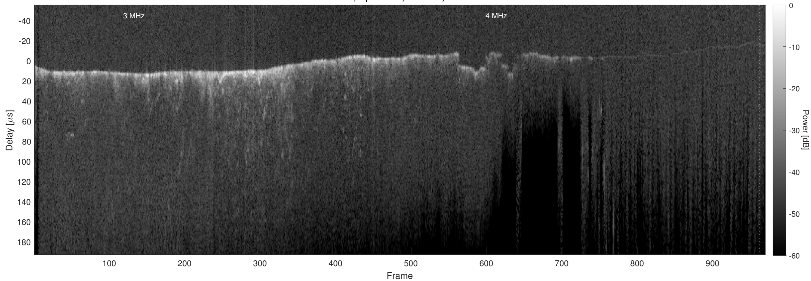
Orbit 9439, Optimized, Window, Channel 2
