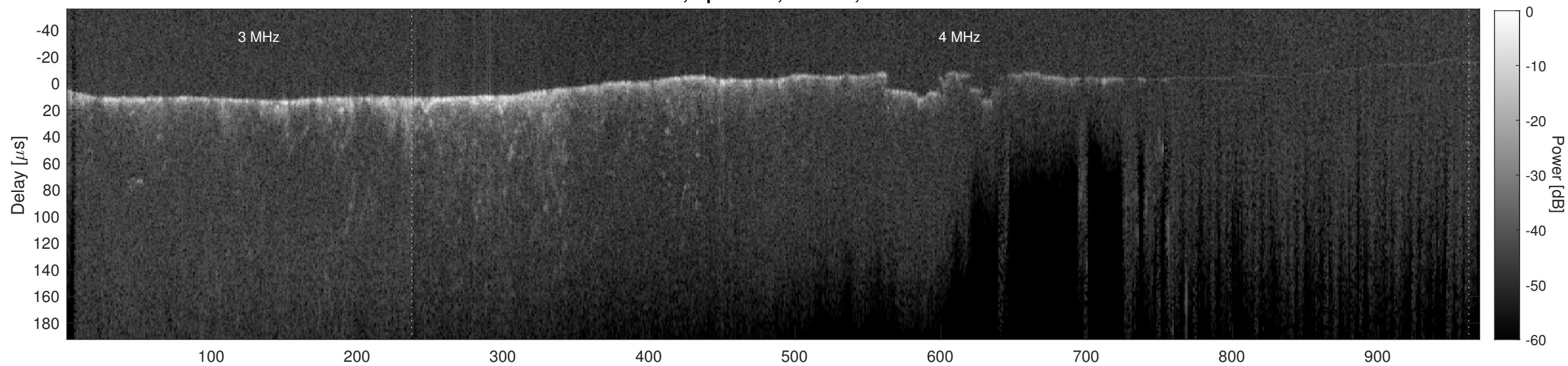
Orbit 9439, Cluttergram
