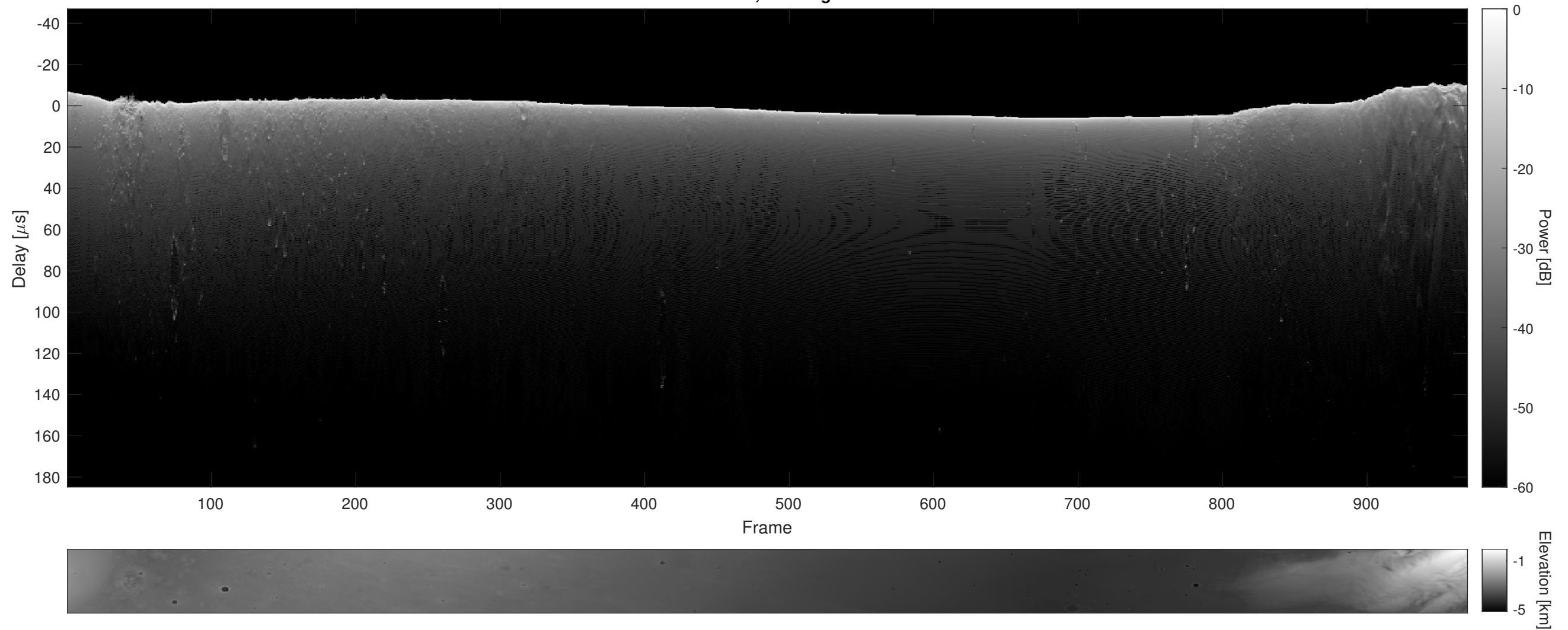
Orbit 9440, Cluttergram
