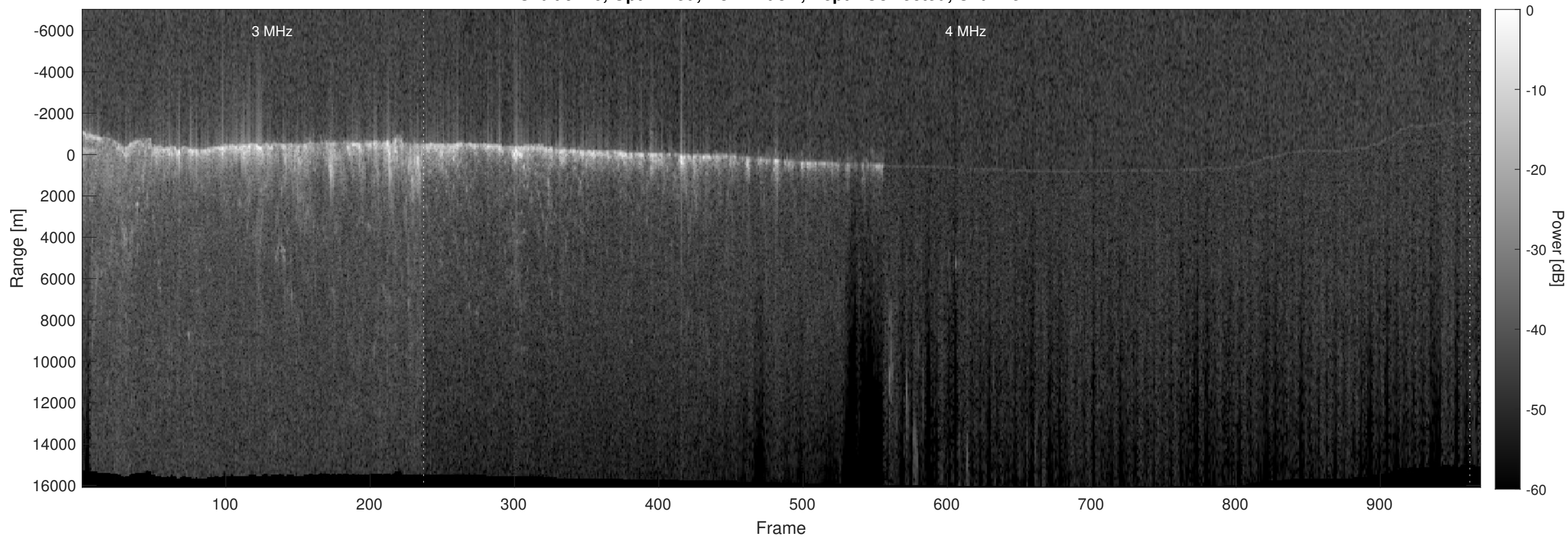
Orbit 9440, Optimized, No Window, Depth-Corrected, Channel 2
